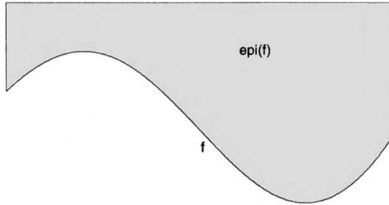
Figure 7.7. The epigraph of a one-dimensional function.
