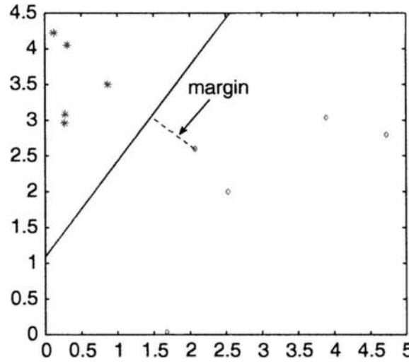
Figure 8.2. The optimal linear separator and its margin.
