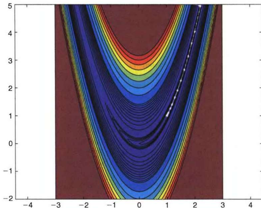
Figure 5.1. Contour lines of the Rosenbrock function along with the 18 iterates of the hybrid Newton's method.
