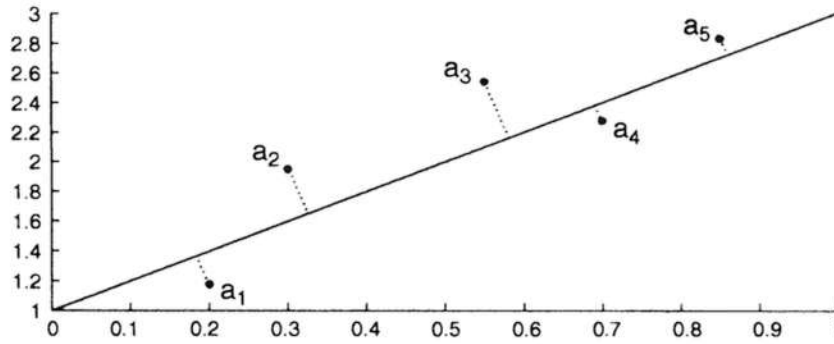
Figure 10.3. A two-dimensional example: given 5 points a_1, \dots, a_5 in the plane, the orthogonal regression problem seeks to find the line for which the sum of squared norms of the dashed lines is minimal.
