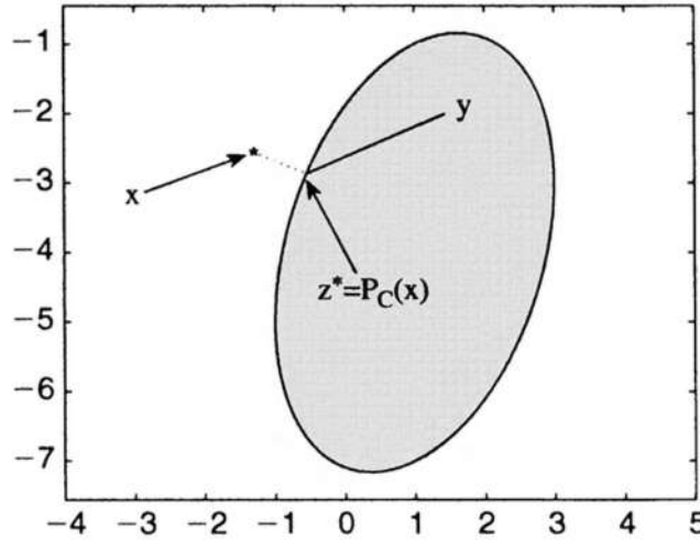
Figure 9.1. The orthogonal projection operator.
