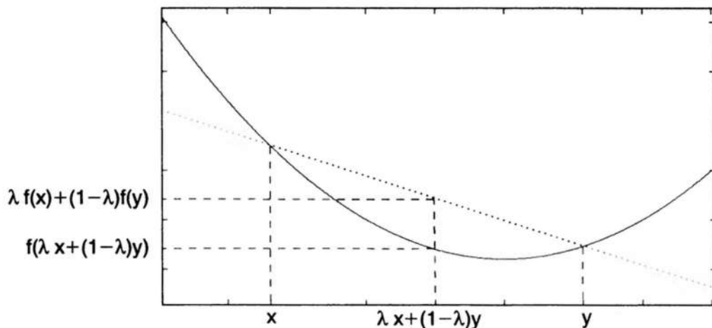
Figure 7.1. Illustration of the inequality f(\lambda \mathbf{x} + (1 - \lambda)\mathbf{y}) \leq \lambda f(\mathbf{x}) + (1 - \lambda)f(\mathbf{y}) .
