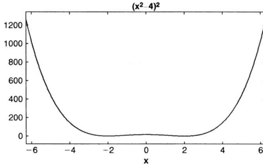
Figure 7.4. The nonconvex function (t^2 - 4)^2 .
