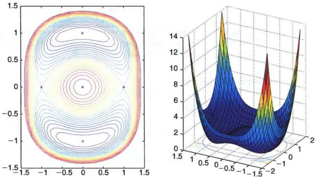
Figure 2.3. Contour and surface plots of f(x_1, x_2) = (x_1^2 + x_2^2 - 1)^2 + (x_2^2 - 1)^2 . The five stationary points (0, 0), (0, 1), (0, -1), (1, 0), (-1, 0) are denoted by asterisks. The points (0, -1), (0, 1) are strict local minimum points as well as global minimum points, (0, 0) is a local maximum point, and (-1, 0), (1, 0) are saddle points.
