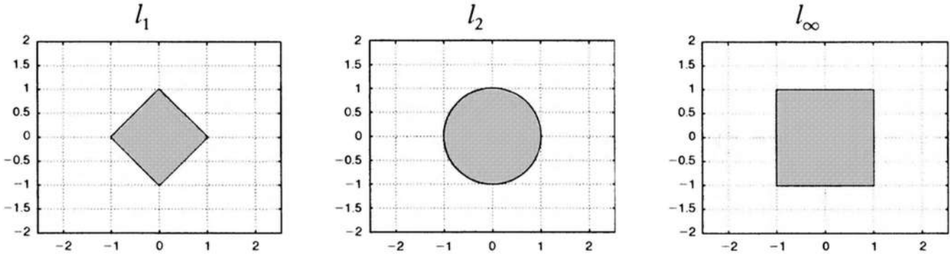
Figure 6.2. l_1 , l_2 , and l_\infty balls in \mathbb{R}^2 .
