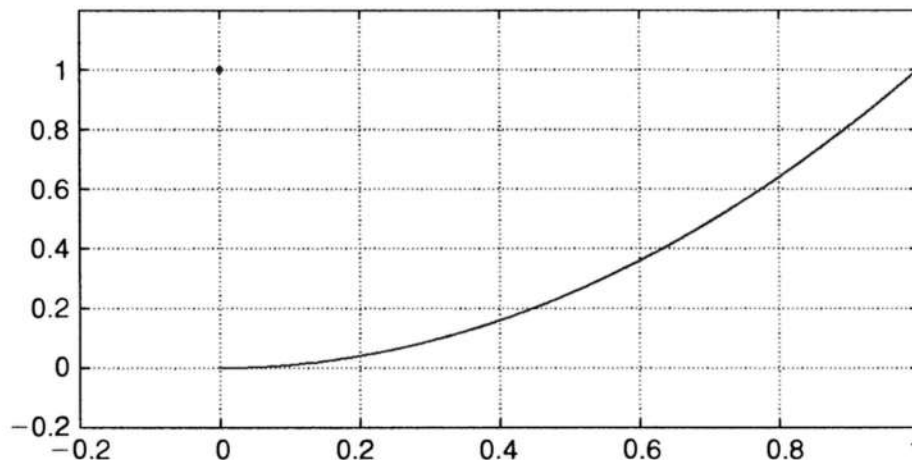
Figure 7.6. A noncontinuous convex function over the interval [0, 1] .
