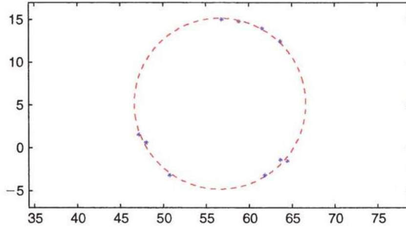
Figure 3.4. The best circle fit (the optimal solution of problem (3.6)) of 10 points denoted by asterisks.
