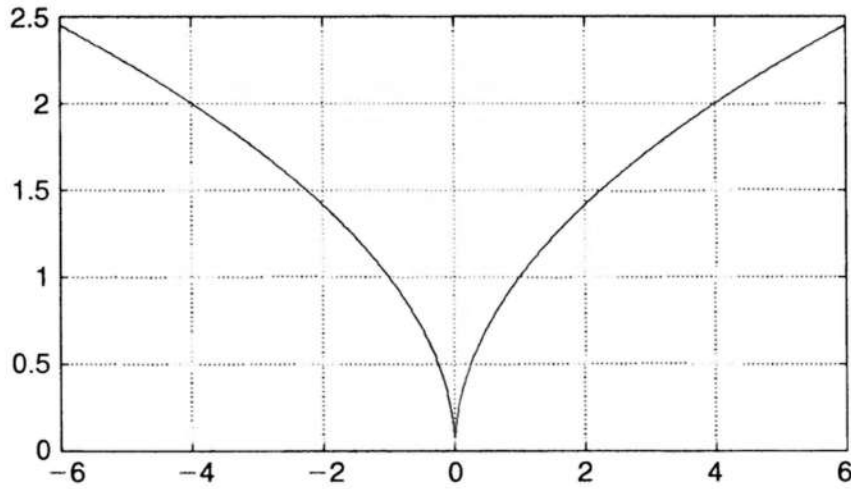
Figure 7.5. The quasi-convex function \sqrt{|x|} .
