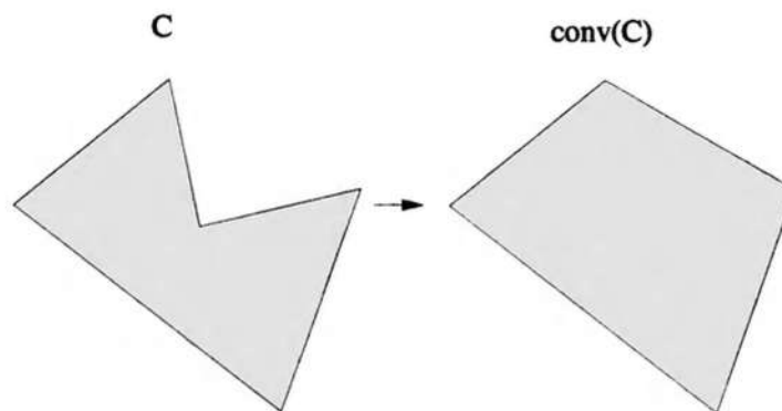
Figure 6.3. A nonconvex set and its convex hull.
